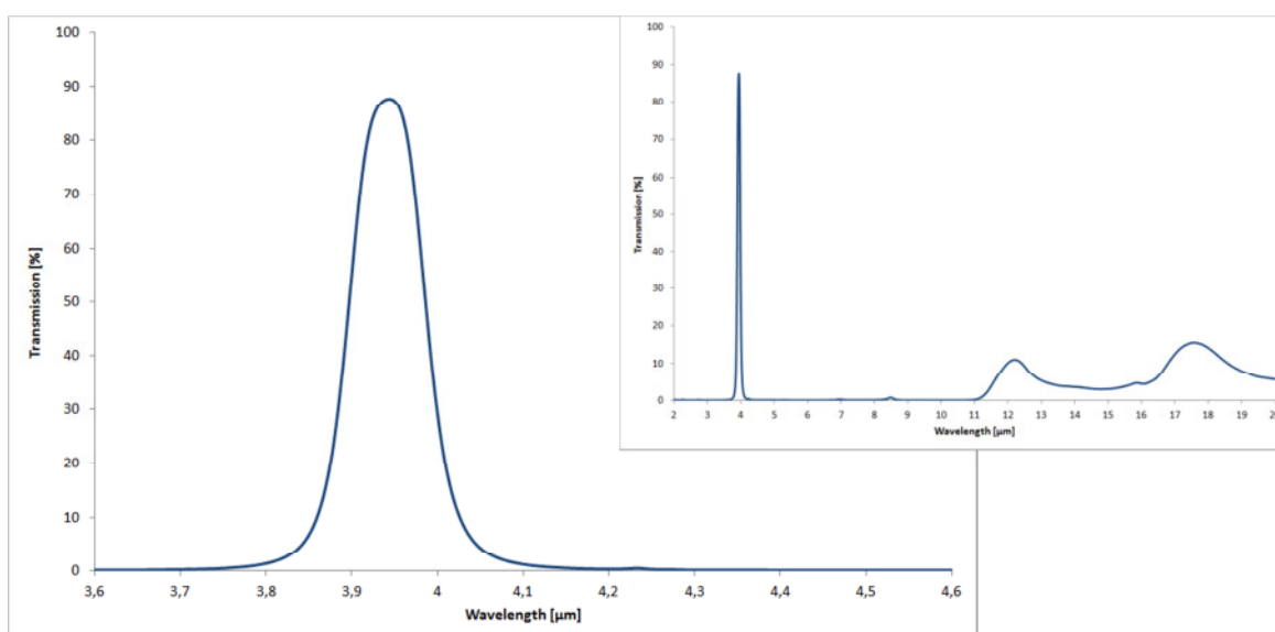
Figure 3 Typical Transmission Characteristics of Filter G20
