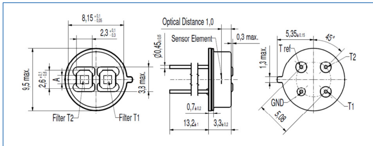
Figure 5 Mechanical drawing of detector TPD 2T 0625 (Drawing No.: 2/71833-0)
