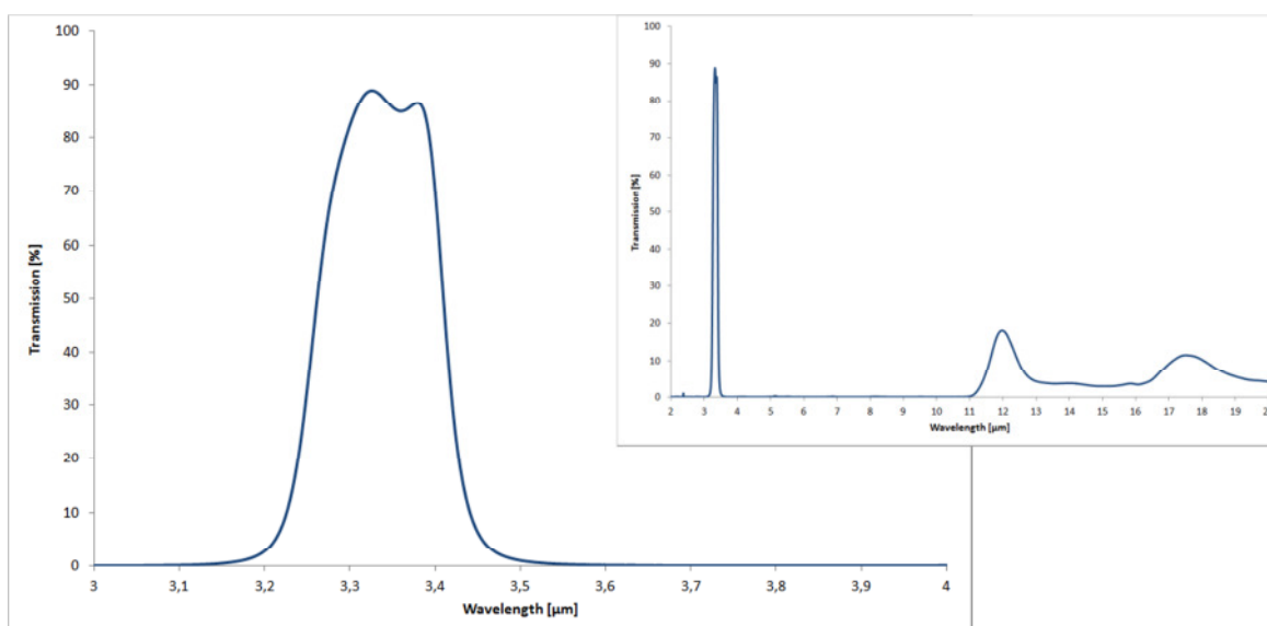
Figure 4 Typical Transmission Characteristics of Filter G5.2
